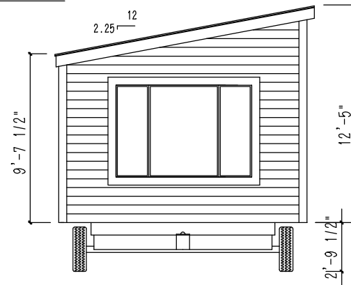
ROADSIDE ELEVATION
